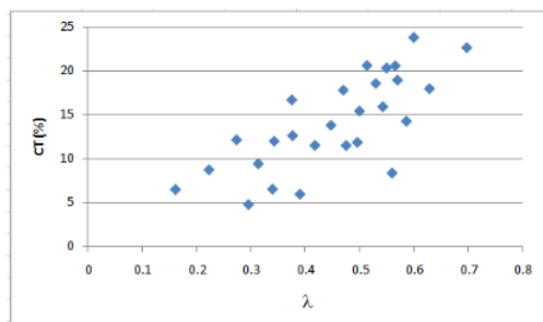
Gambar 7. Variasi Ct terhadap tip speed ratio
